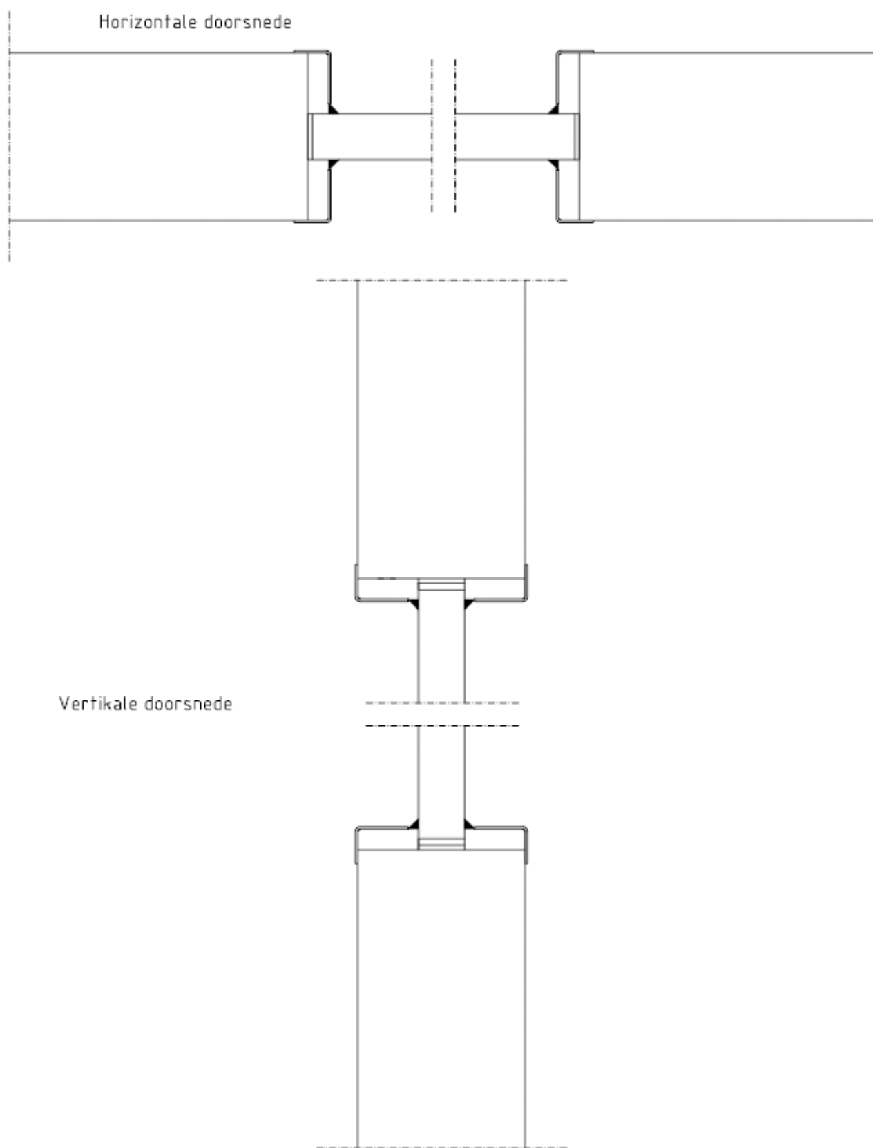
Fig. 4c : Brandwerende beglazing
