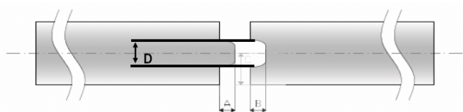
Figure 1 – Rainure et languette
