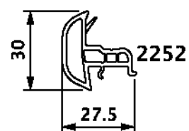
Figure 1i – Profilés de finition (suite)
