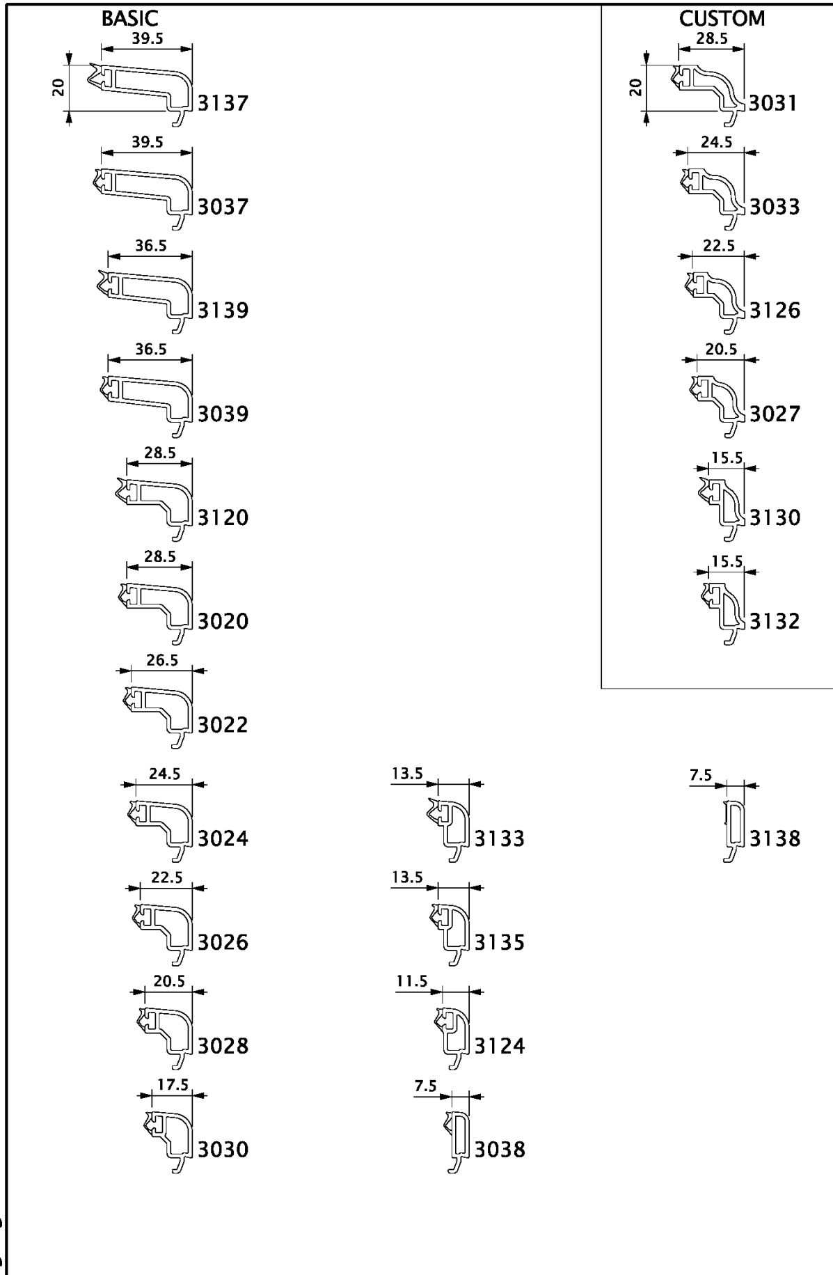
Figure 1g – Parcloses
