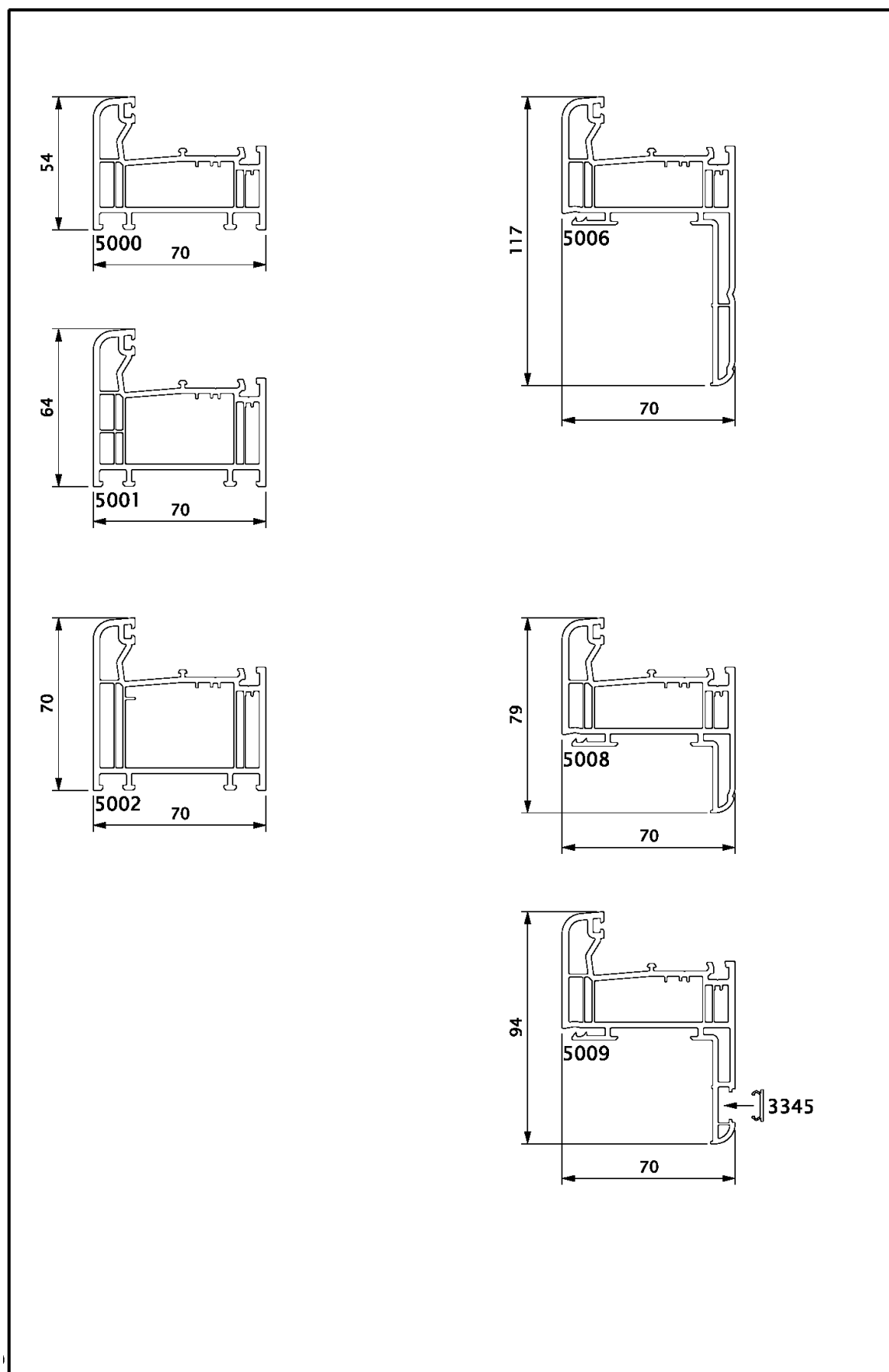
Figure 1a – Profilés dormants (suite)
