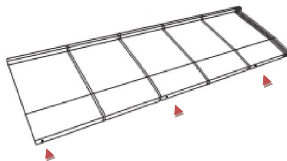
Fig. 13: tuile DECRA® QUADRO (ACOUSTIC) BY ICOPAL – position des fixations
