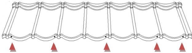
Fig. 6: tuile DECRA® CLASSIC, DECRA® ELEGANCE – position des fixations
