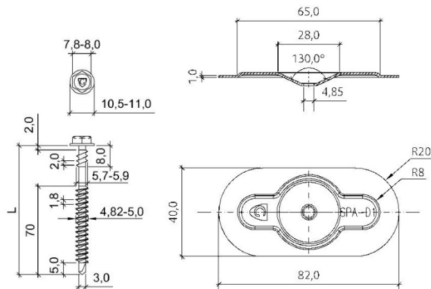
Fig. 2 – vis GUARDIAN® DBT(A) 4,8 + plaque GUARDIAN® SPA 82x40
