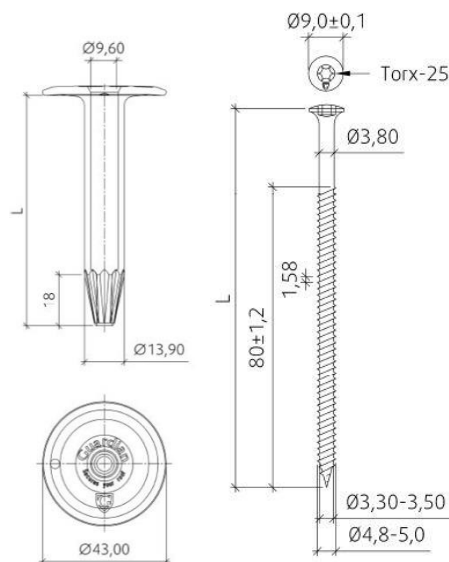
Fig. 3 – Systeem GUARDIAN RP45 – PS48
