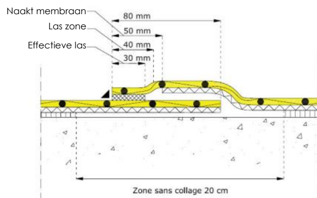
Fig. 1 – Overlapverbindingen (langsrichting)
