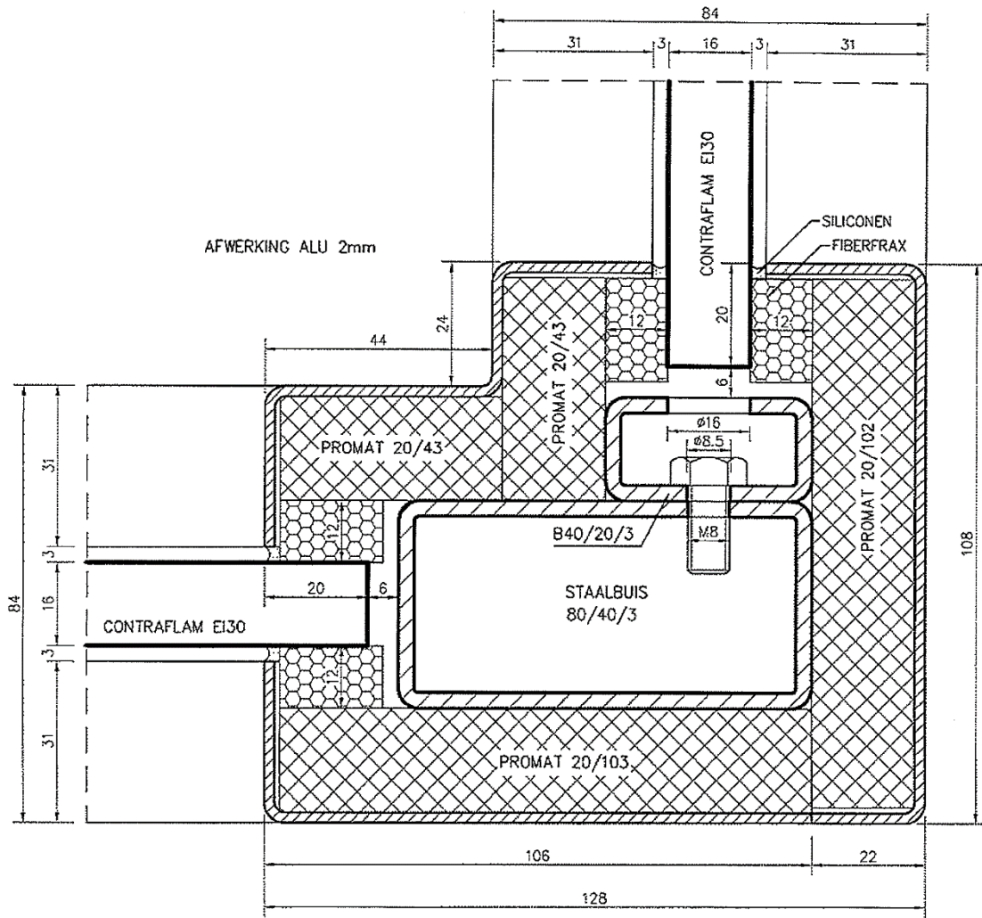
Detail 14: Hoekverbinding raam (rechte hoek) - variante
