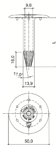
Fig. 7 – Schroef GUARDIAN BS48
