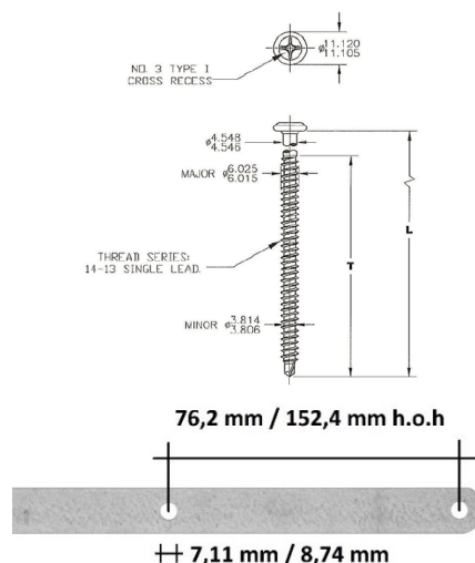
Fig. 1 – Elevate Schroef "ALL PURPOSE FASTENER" + bevestigingsstrip "Metal Batten Strip"
