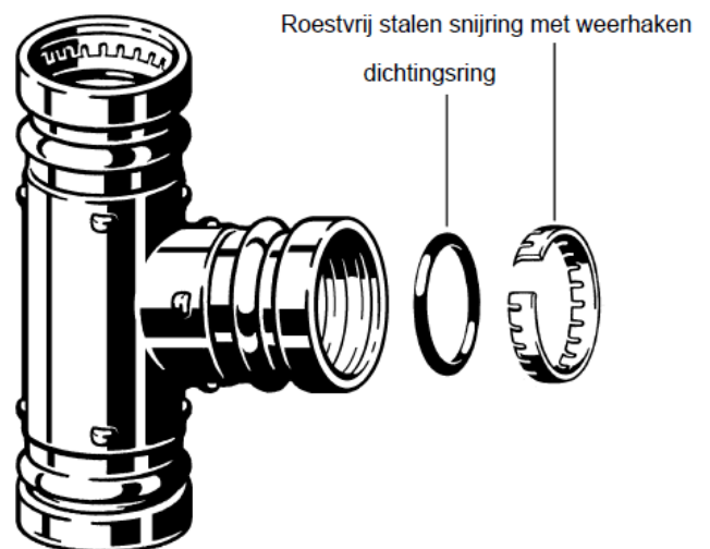
Fig. 2: Profipress XL
