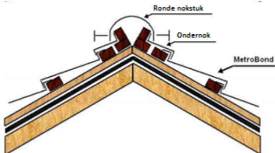
Fig. 27– METROTILE® BOND, METROTILE® BOND 7-PA, METROTILE® ROMAN, METROTILE® CLASSIC, METROTILE® SHAKE, METROTILE® WOODSHAKE, METROTILE® MISTRAL, METROTILE® MISTRAL, METROTILE® ROMANA, METROTILE® GALLO, METROTILE® ELEGANTA dakpan – halfrond nokstuk
