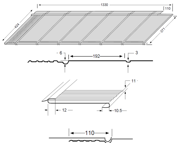
Fig. 13- METROTILE® I-PANEL dakpan
