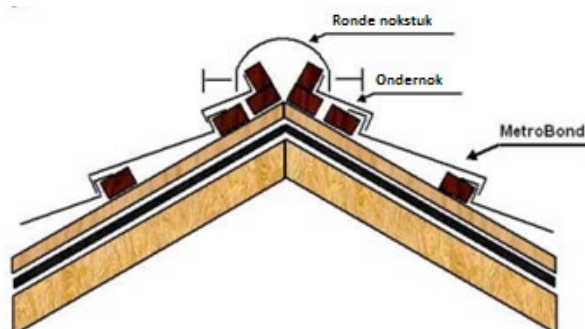
Fig. 33– METROTILE® shingle, METROTILE® VIKSEN, METROTILE® I-SHAKE, METROTILE® I-PANEL, METROTILE® I-SLATE en METROTILE® I-SHINGLE dakpan – half rond nokstuk
