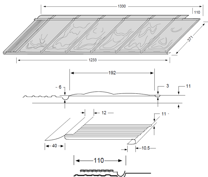
Fig. 14- METROTILE® I-SLATE dakpan
