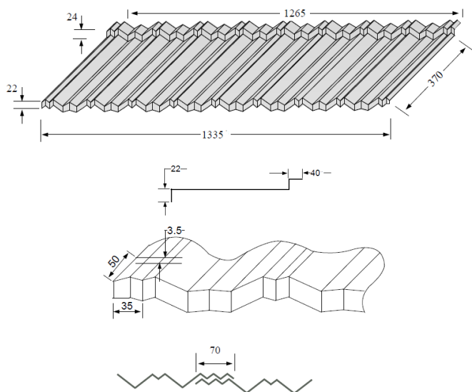
Fig. 4– METROTILE® CLASSIC dakpan
