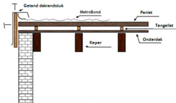
Fig. 28– METROTILE® BOND, METROTILE® BOND 7-PA, METROTILE® ROMAN, METROTILE® CLASSIC, METROTILE® SHAKE, METROTILE® WOODSHAKE, METROTILE® MISTRAL, METROTILE® MISTRAL, METROTILE® ROMANA, METROTILE® GALLO, METROTILE® ELEGANTA dakpan – zijrand
