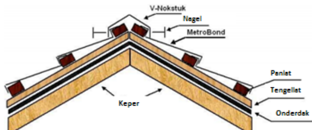
Fig. 26– METROTILE® BOND, METROTILE® BOND 7-PA, METROTILE® ROMAN, METROTILE® CLASSIC, METROTILE® SHAKE, METROTILE® WOODSHAKE, METROTILE® MISTRAL, METROTILE® MISTRAL, METROTILE® ROMANA, METROTILE® GALLO, METROTILE® ELEGANTA dakpan – V-vormig-nokstuk
