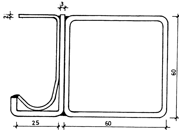
Figure 3 : Rail renforcé
