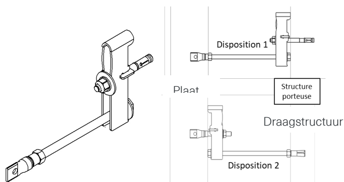
"Open" windverankering
