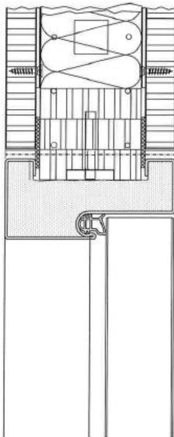
fig.47 – JB
