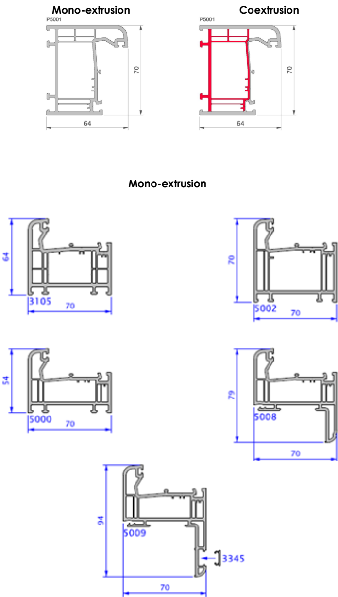
Figure 2a: Profilés dormants
