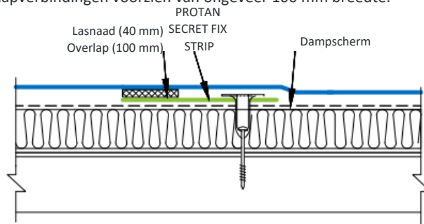
Fig. 14 – Overlapverbindingen (PROTAN SECRET FIX STRIP)
