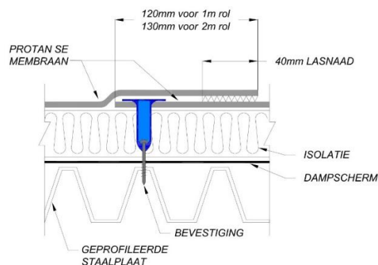
Fig. 13 – Overlapverbindingen (langsrichting)
