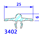
Figure 5.c : Rail coulissant
