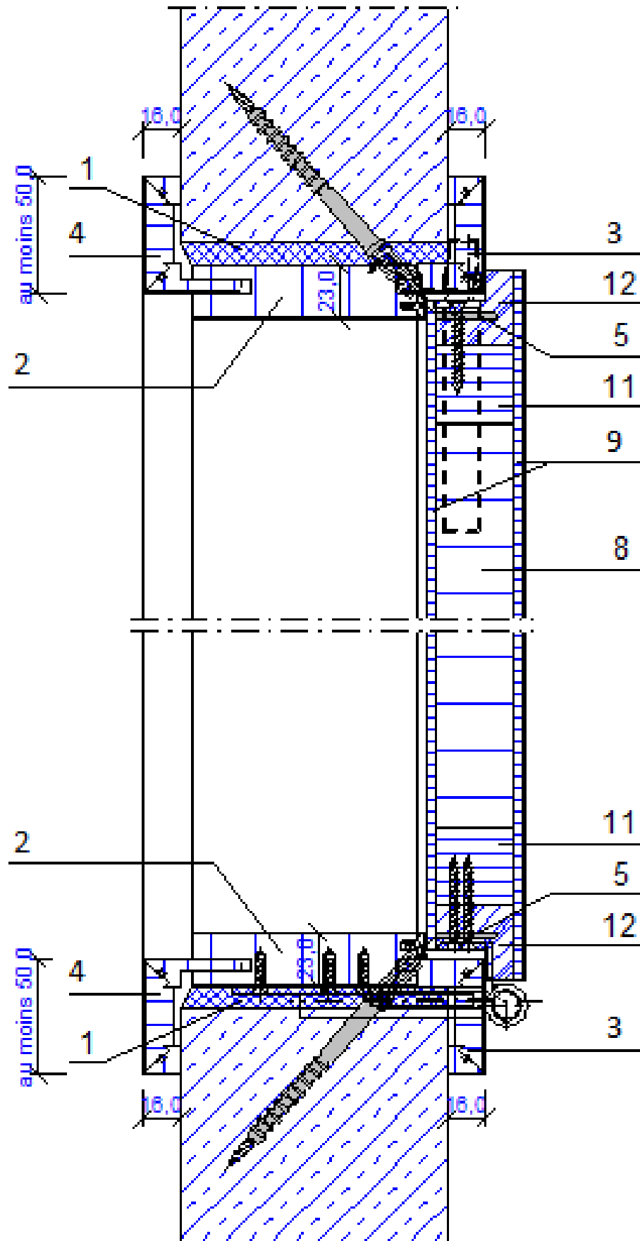
Figure 2 – Coupe horizontale – Type A
