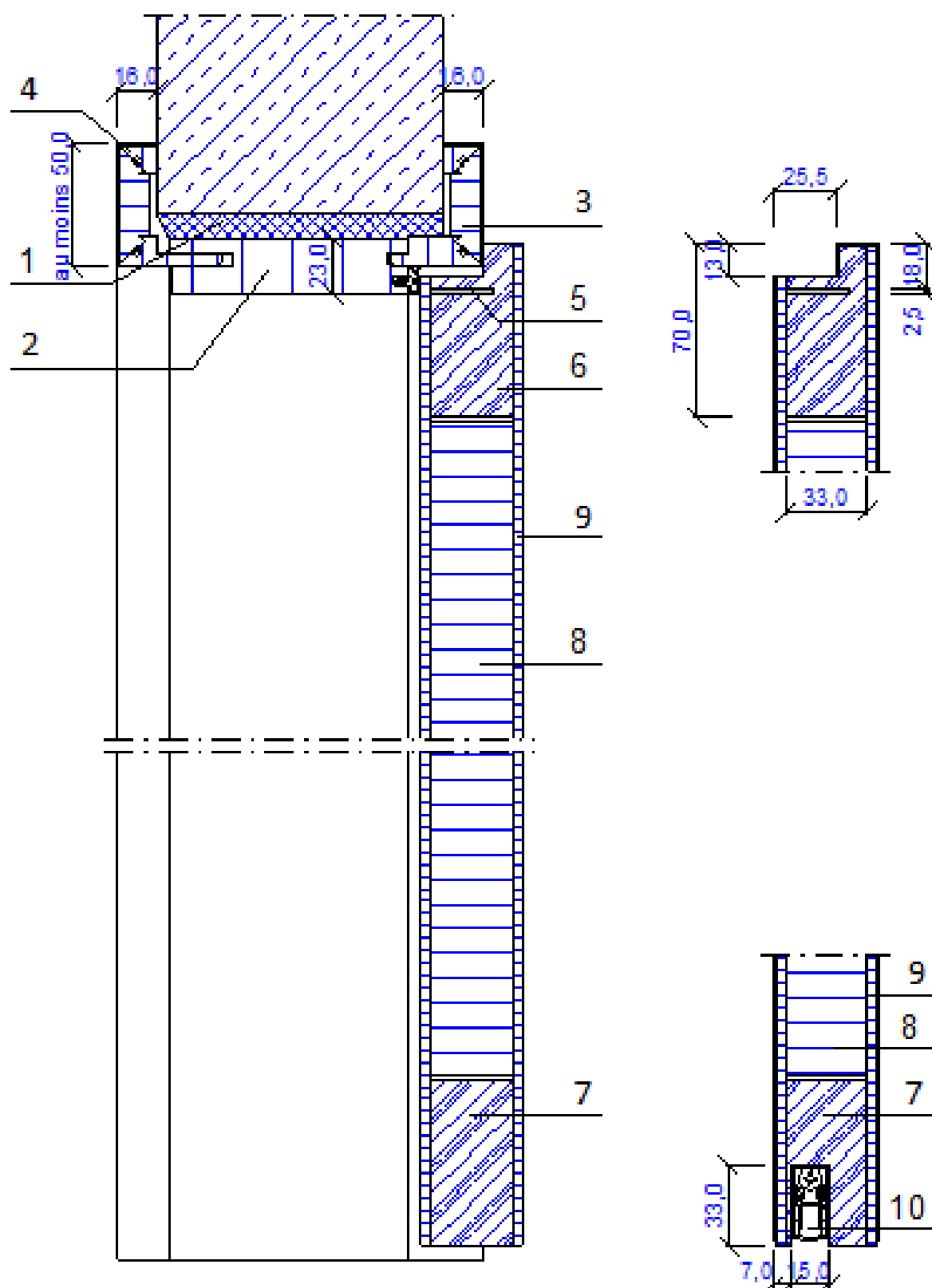
Figure 1 – Coupe verticale – sans imposte – Type A
