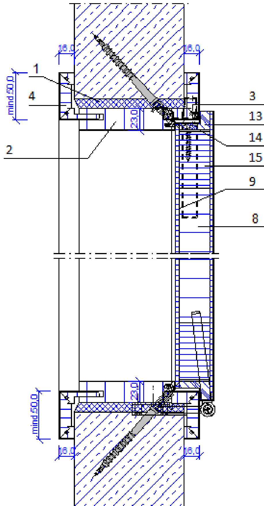
Figure 4 – Coupe horizontale – Type B
