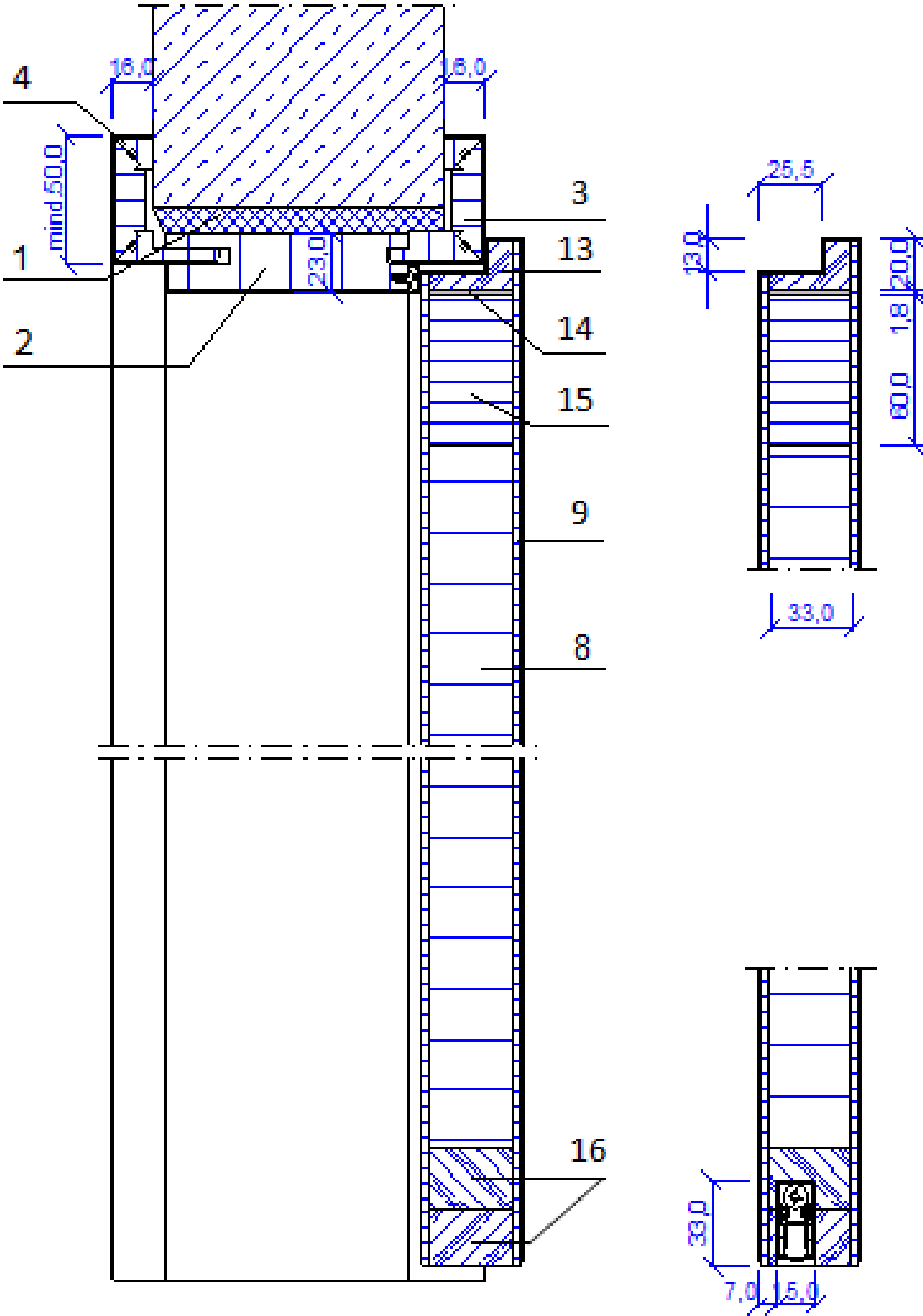
Figure 3 – Coupe verticale – sans imposte – Type B
