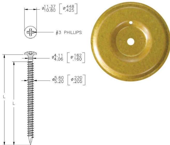
Fig. 8 – OMG 80mm RHINOBOND INSULATION PLATE + OMG #12 STANDARD ROOFGRIP schroef
