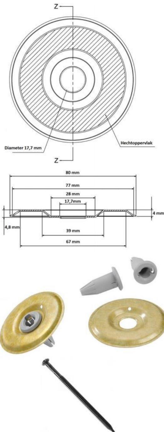
Fig. 7 – OMG RHINOBOND TREADSAFE PLATE (boven) + OMG XHD (Extra Heavy Duty) schroef (onder) + OMG TREADSAFE TULE (onder)
