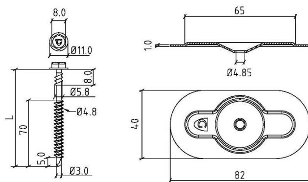
Fig. 4 – Vis GUARDIAN DBT(A) 4,8 + plaquette GUARDIAN SPA 8240
