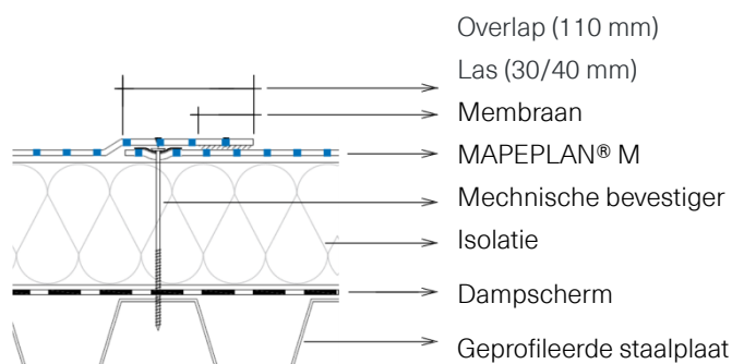
Fig. 9 – Overlapverbindingen (langsrichting)
