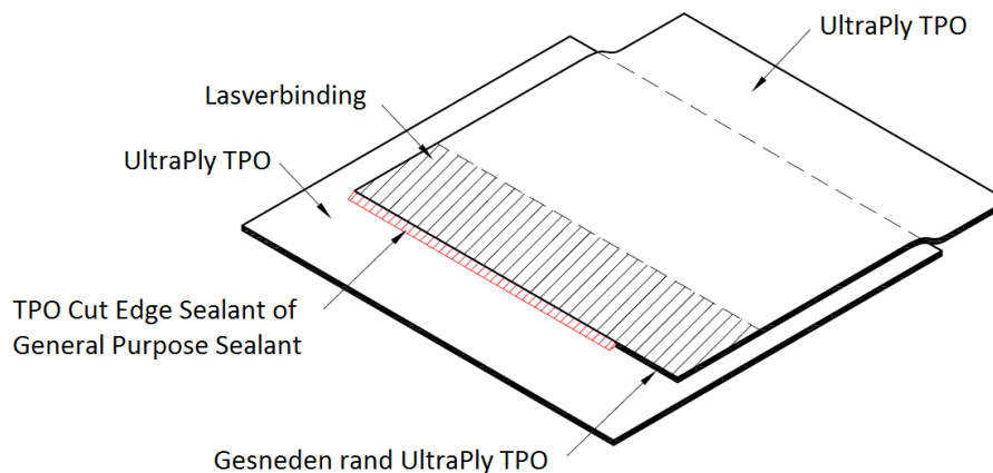
Fig. 19 – overlapverbindingen
