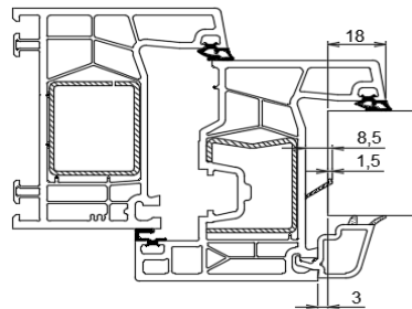
Figuur 10 - Convectionsscheiding in de glasspunningbodem
