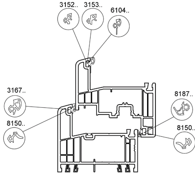
Figure 4 : Joints
