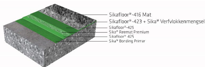
Fig. 6– SIKAFLOOR® MONOFLEX DECO+ BALCONY SYSTEM
