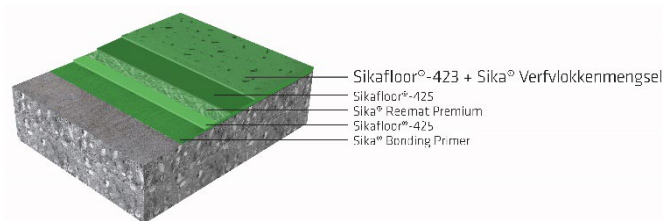
Fig. 3– SIKAFLOOR® MONOFLEX DECO BALCONY SYSTEM
