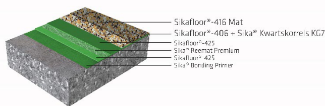
Fig. 4– SIKAFLOOR® MONOFLEX QUARTZ BALCONY SYSTEM
