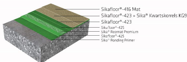
Fig. 5– SIKAFLOOR® MONOFLEX SOLID FINE BALCONY SYSTEM
