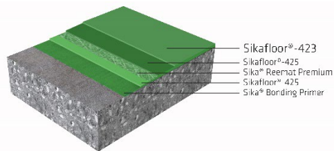
Fig. 7– SIKAFLOOR® MONOFLEX UNI BALCONY SYSTEM
