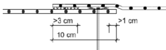
Figuur 1: – Overlapverbindingen
