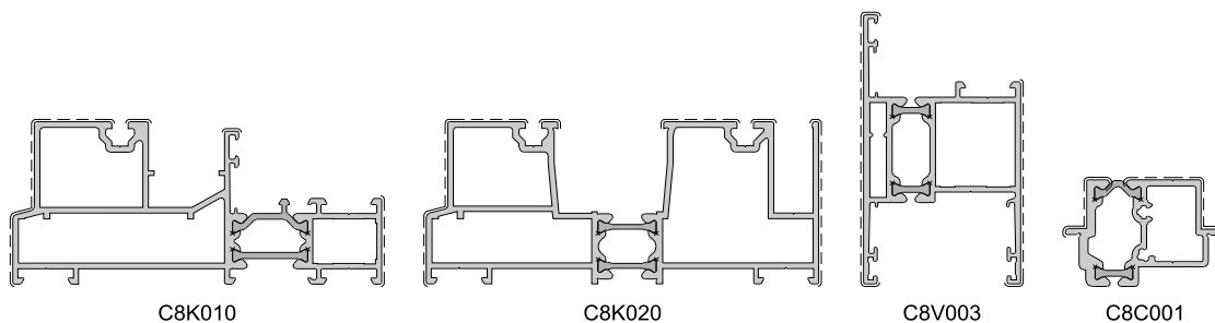
Figure 3 : Confort 125 - Confort 130
