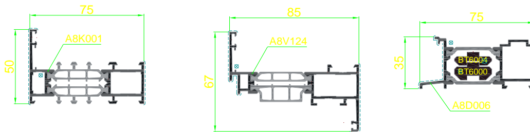
Figure 8 –Avantis 75
