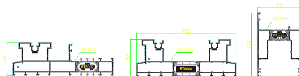
Figure 4 - Confort 160 - Smartline
