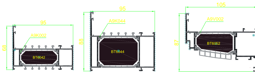
Figure 10 – Avantis 95
