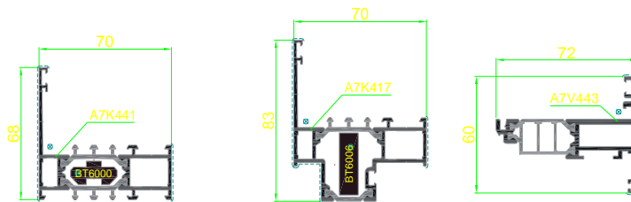
Figure 7 –Avantis 70HV
