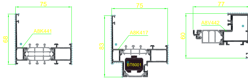
Figure 9 –Avantis 75HV
