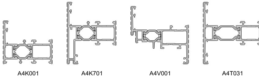
Figure 6 –Avantis 70
