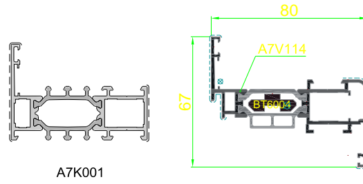
Figure 6 –Avantis 70
