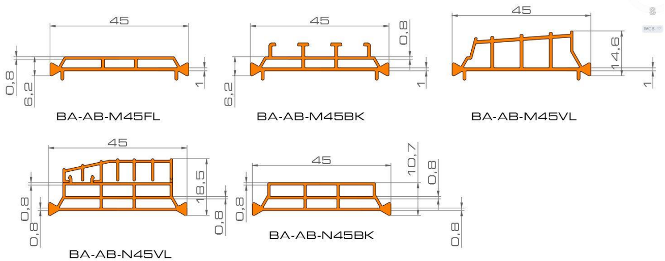
Figure 8: Système Triton
