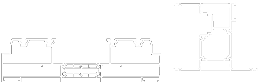
Figure 5 – MB-77HS
