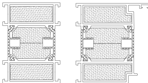
Figure 6 – MB-78EI
