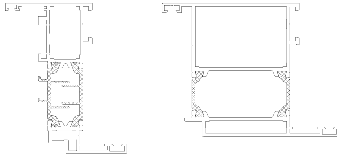
Figure 3 – MB-70B
