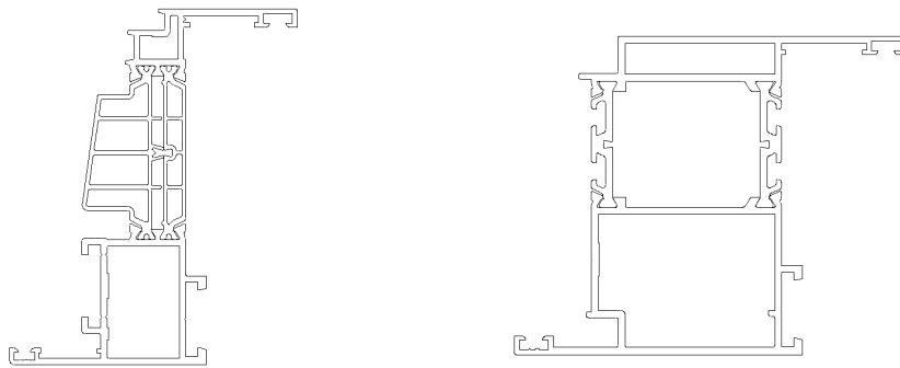
Figure 5 – MB-77HS
