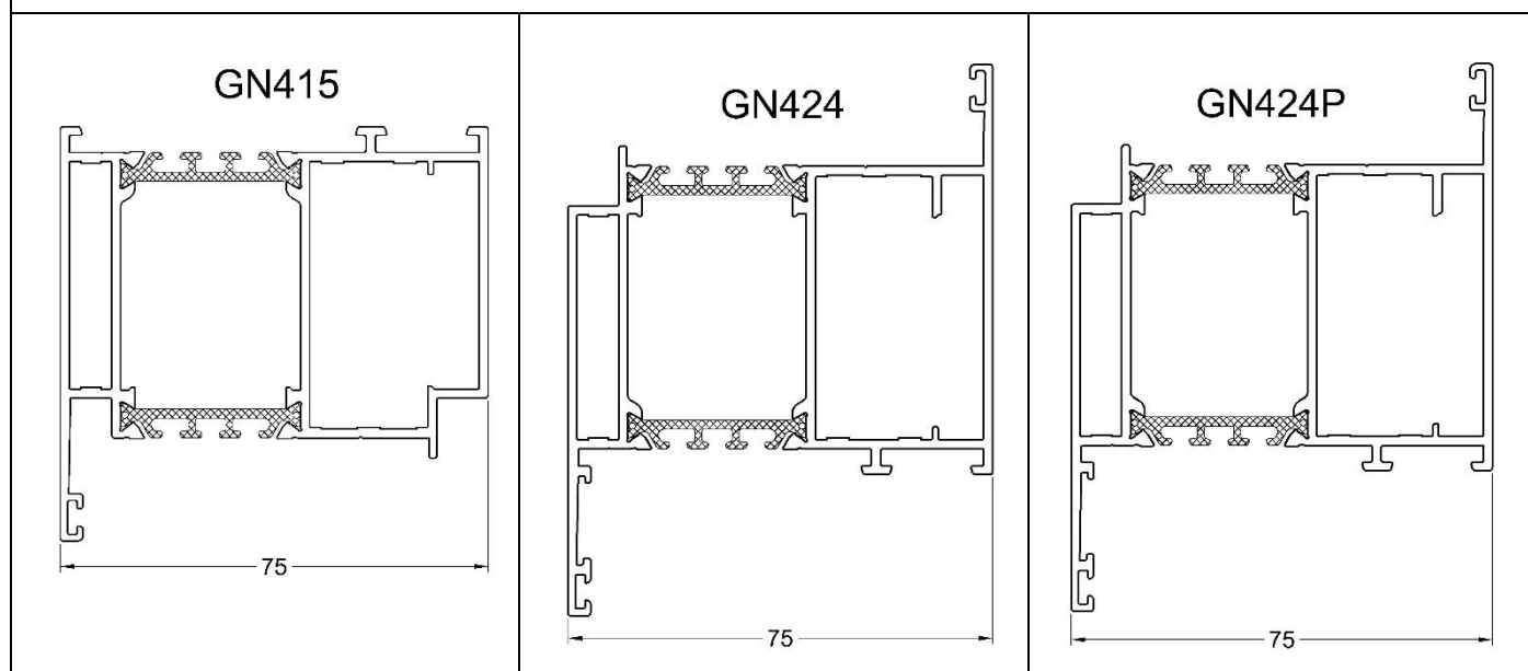
Figure 4 – Exemple Aliplast Genesis 75 portes
