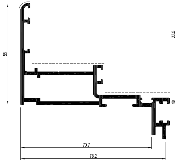
Frame: 034.1121.XX
