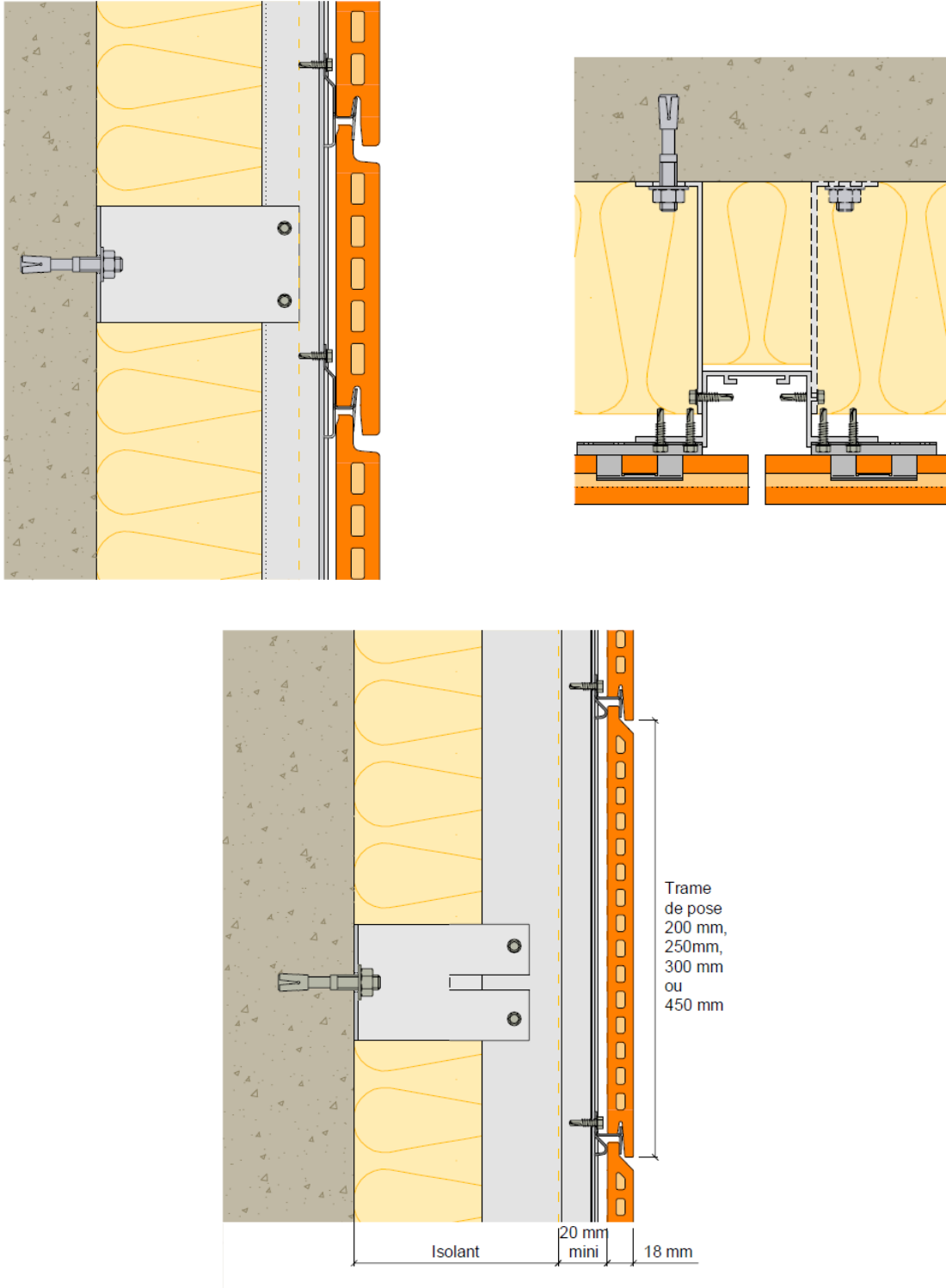
Figure 3: typical installation details (U-section)
