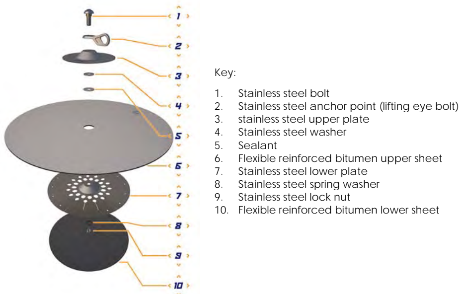
Figure 1 - Build-up of the assembled structural anchor
