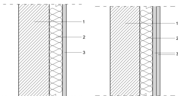
Figure 1: The assessed constructions for airborne sound insulation
